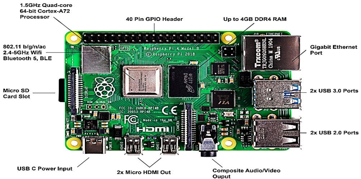
Fig 2. Raspberry Pi Model B.
