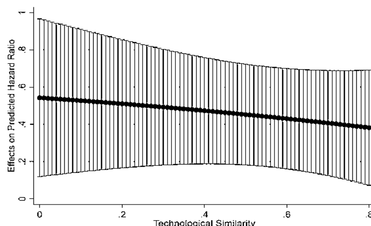
Fig 1. Interaction Effect Between Technical Similarity and Primary Competitors of Ecosystem Investors
