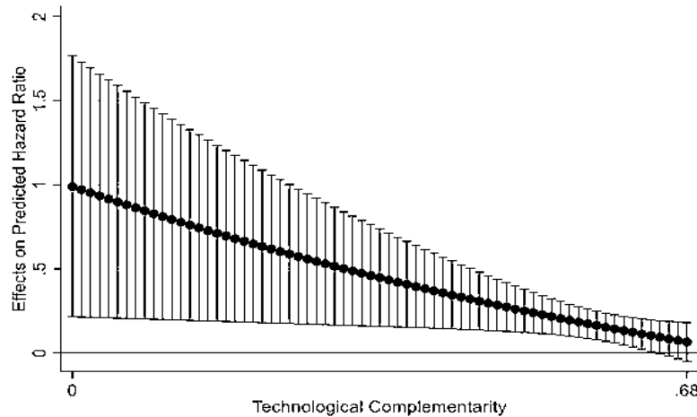
Fig 2. Interaction Impact Between Alliances with Main Ecosystem Investors and Technical Complementarity Verification of Results
